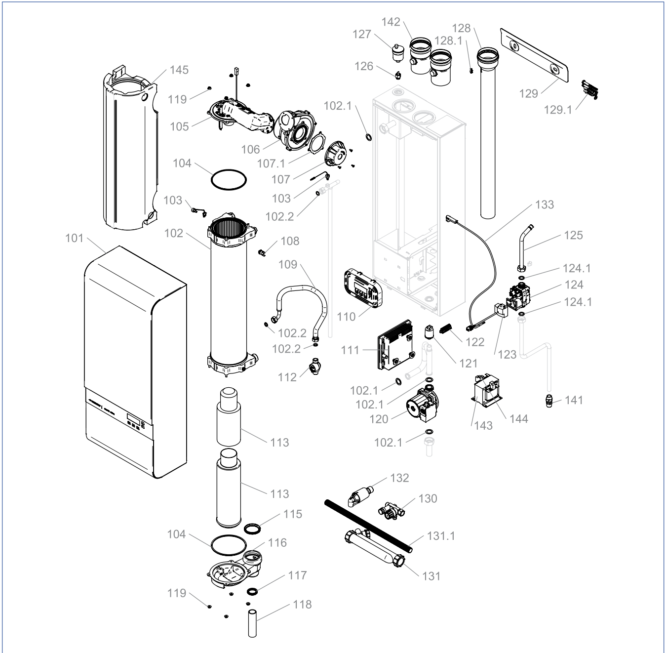
Exploded view
